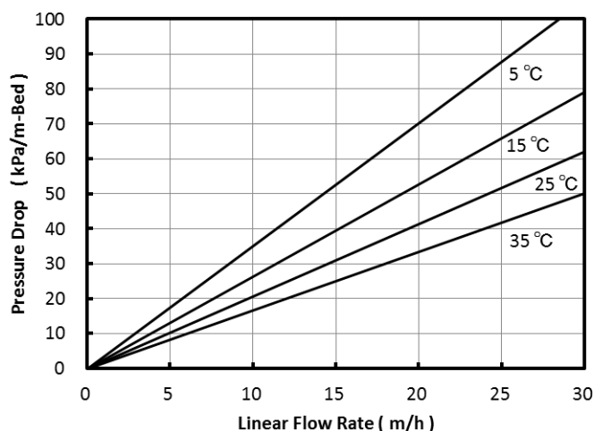
Fig. 1 Pressure Drop of UBK535K
