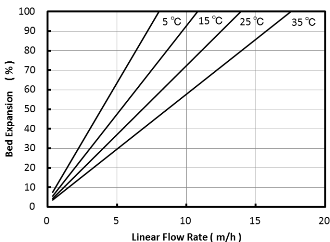
Fig. 2 Bed Expansion of UBK535K
