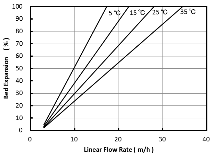
Fig. 2 Bed Expansion of PK216L
