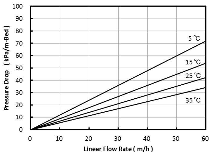
Fig. 1 Pressure Drop of PK216L
